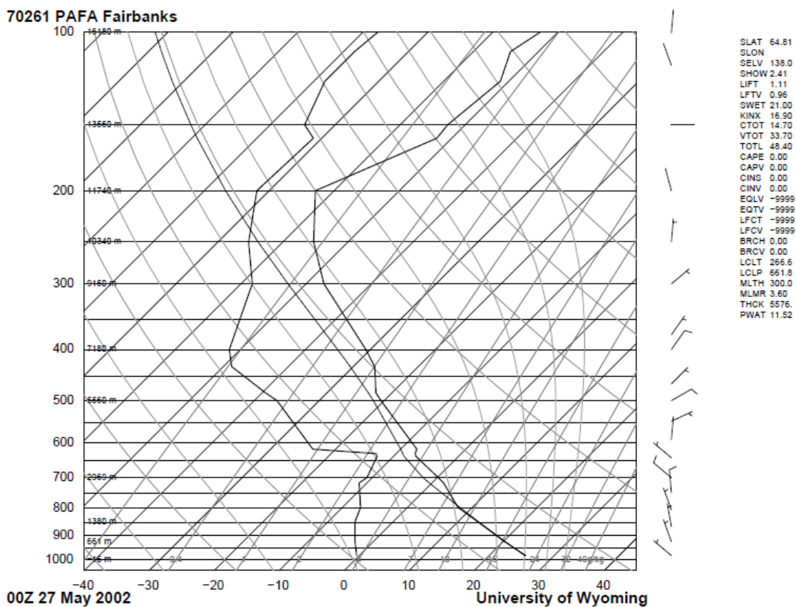
Figure 26. Skew-T chart for Fairbanks at 00 UTC 27 May 2002. There is a mixed layer approximately 4,000 m deep with a thin, more stable layer on top. The air mass was quite dry. The high temperature that day was 27°C. The minimum relative humidity for the day was 18%. The alder pollen count on that day was 623 grains/m 3 . The spruce pollen count on that day was 2,880 grains/m 3 , the highest count for spruce in Anderson's 23 years of data.
