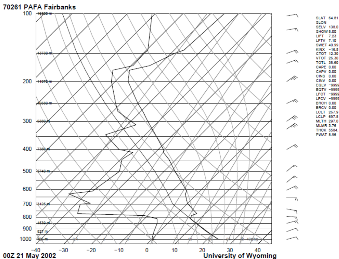
Figure 25. Skew-T chart for Fairbanks at 00 UTC 21 May 2002. There is a mixed layer approximately 2,000 m deep. The temperature inversion just above the mixed layer would limit further upward mixing. The air mass was very dry. The high temperature that day was 27C. The minimum relative humidity for the day was 18%. The birch pollen count on that day was 9,299 grains/m 3 the highest pollen count for any taxon in the 23 years of Anderson's data.
